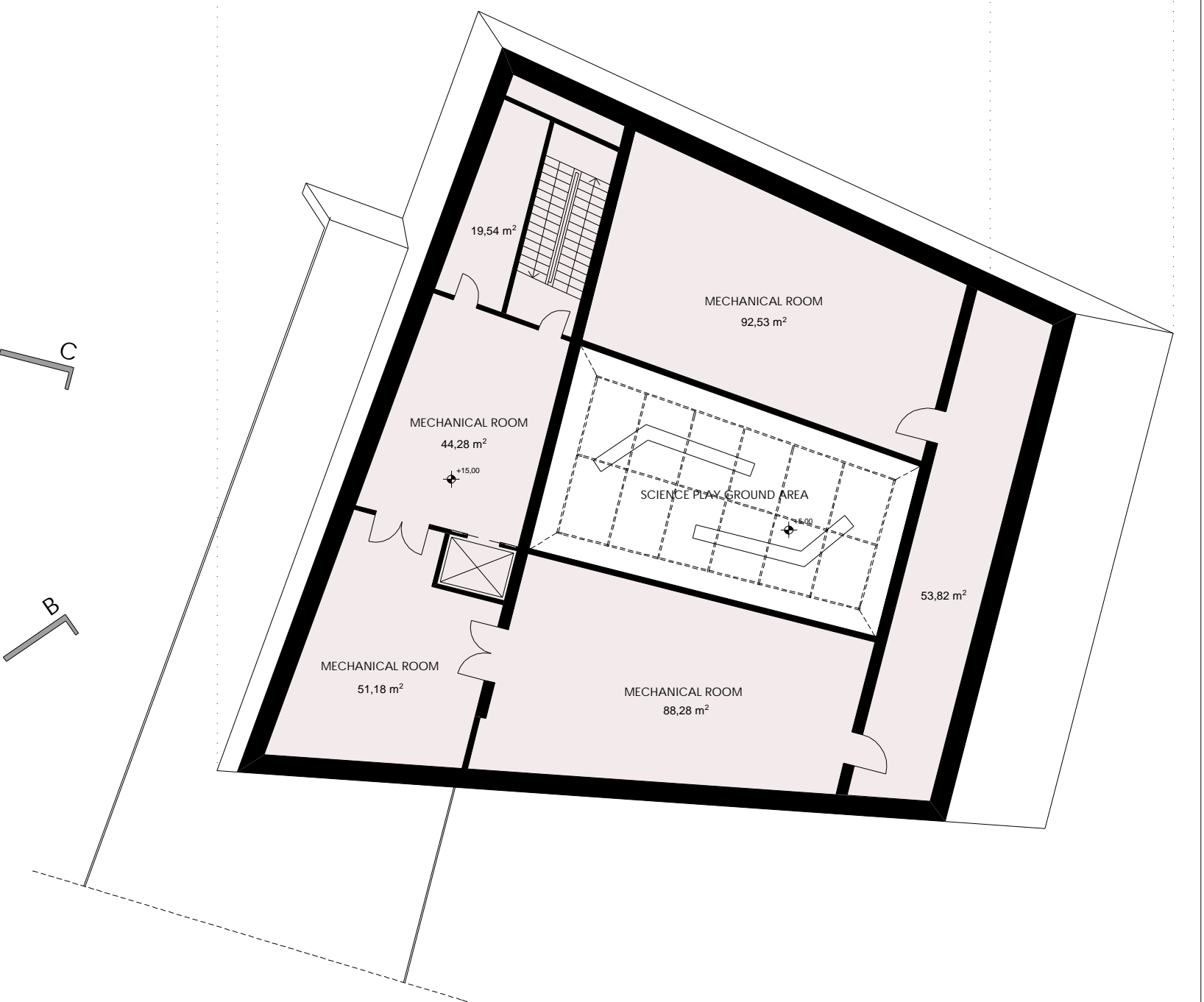
THIRD FLOOR PLAN SCALE-1:200
